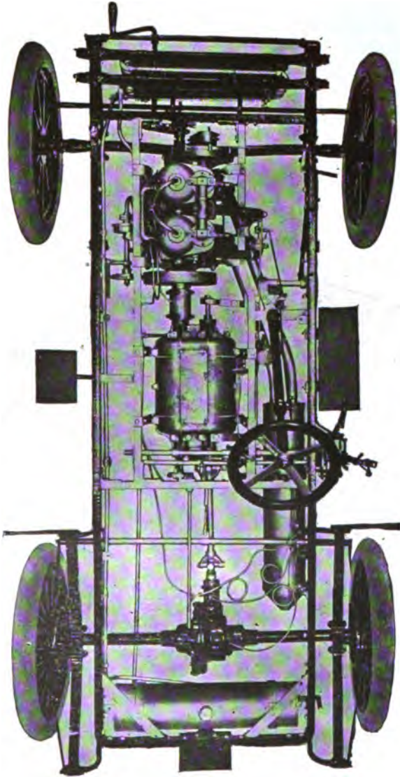
FIG. 409.—Plan of the "Peerless" Carriage, showing position of the motor and mechanism.
